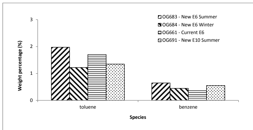
Figure 2. Comparison of toluene and benzene in profiles OG683, OG684, OG661 and OG691
