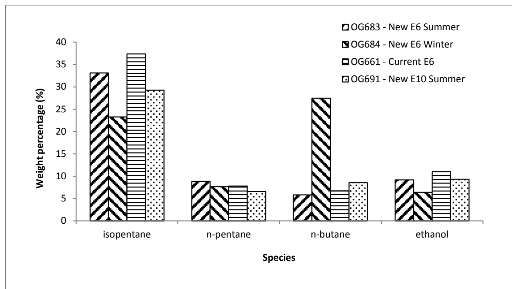
Figure 1. Comparison of major species in profiles OG683, OG684, OG661 and OG691
