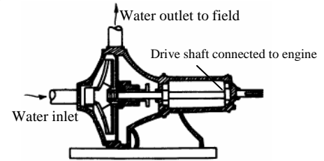
Diagram of centrifugal irrigation pump. Source: Scherer 1993.
