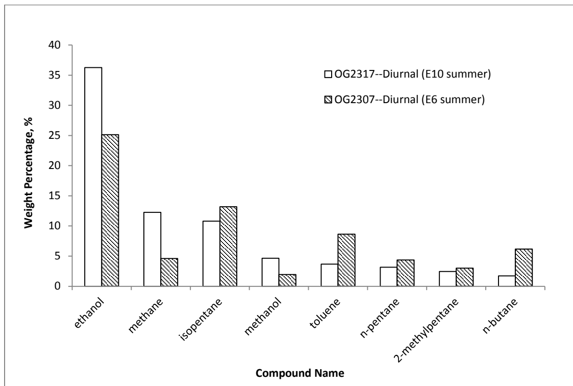
Figure 1. Profile comparison of selected species for OG2317 and OG2307
