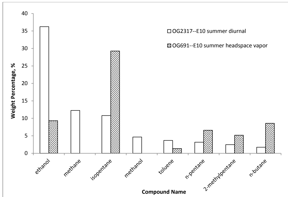
Figure 2. Profile comparison of selected species for OG2317 and OG691
