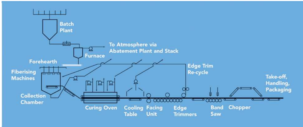
Figure 1. Typical Glass Wool Plant (Rotary Process)
