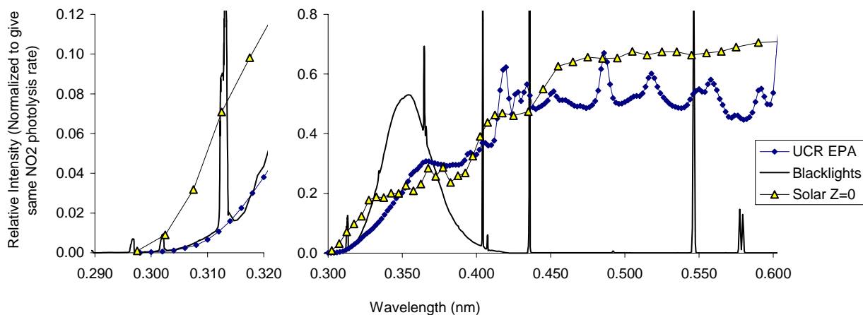
Figure 2. Spectrum of the argon arc light source used in the UCR EPA chamber. Blacklight and representative solar spectra, with relative intensities normalized to give the same NO 2 photolysis rate as that for the UCR EPA spectrum, are also shown.
