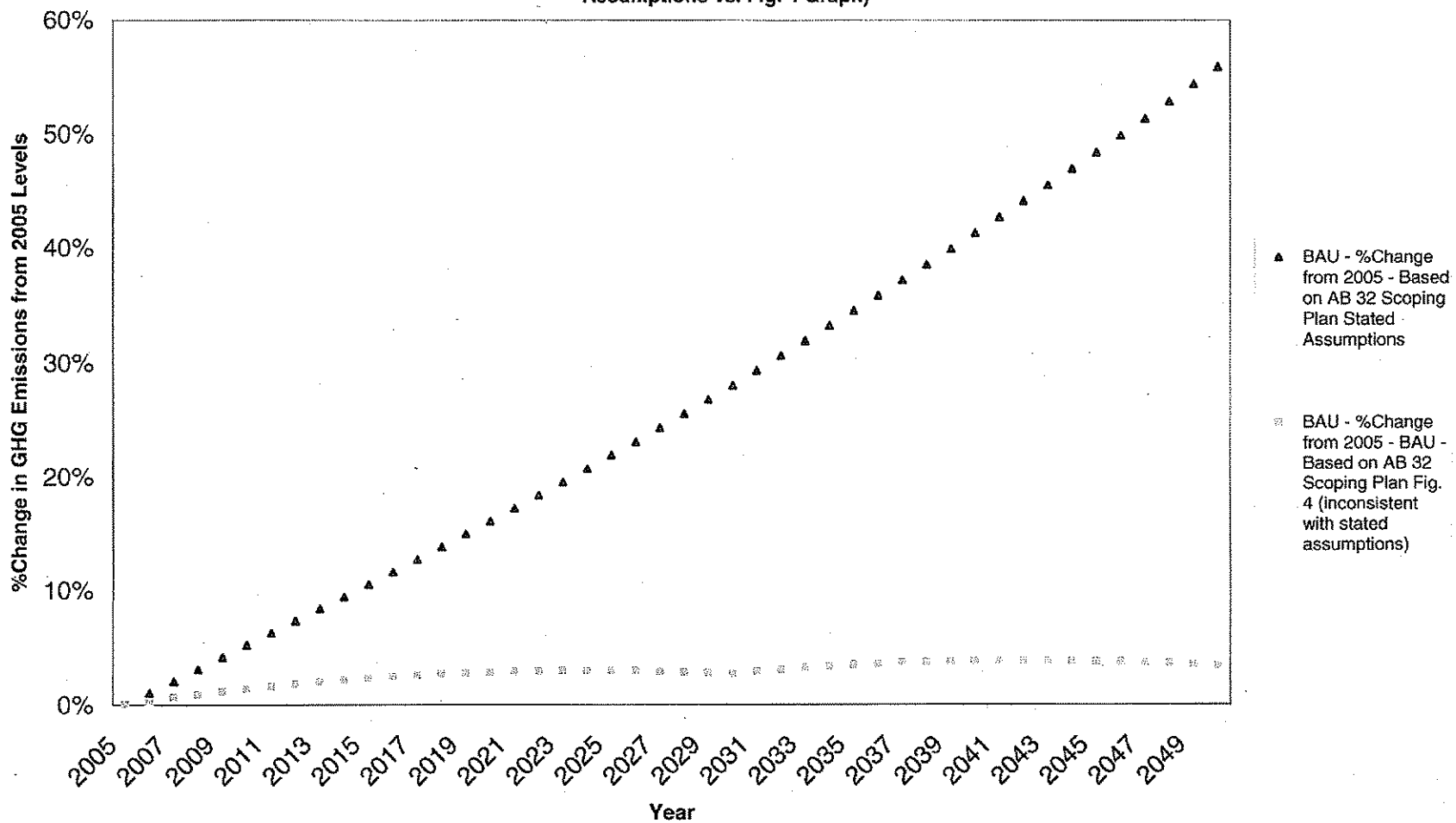
FIGURE 5 Business as Usual Comparison of the Percentage Change in Per Capita GHG Emissions - AB 32 Scoping Plan (Stated Assumptions vs. Fig. 4 Graph)
