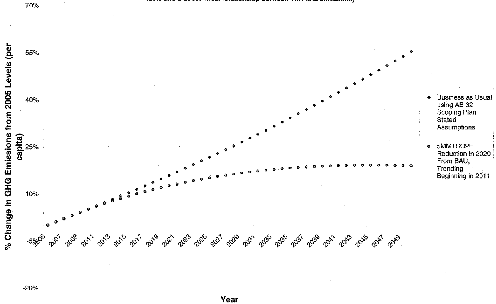
FIGURE 6 Percentage Change in Per Capita GHG Emissions - AB 32 Scoping Plan (Stated Assumptions, assuming 2005 vehicles and fuels and a direct linear relationship between VMT and emissions)
