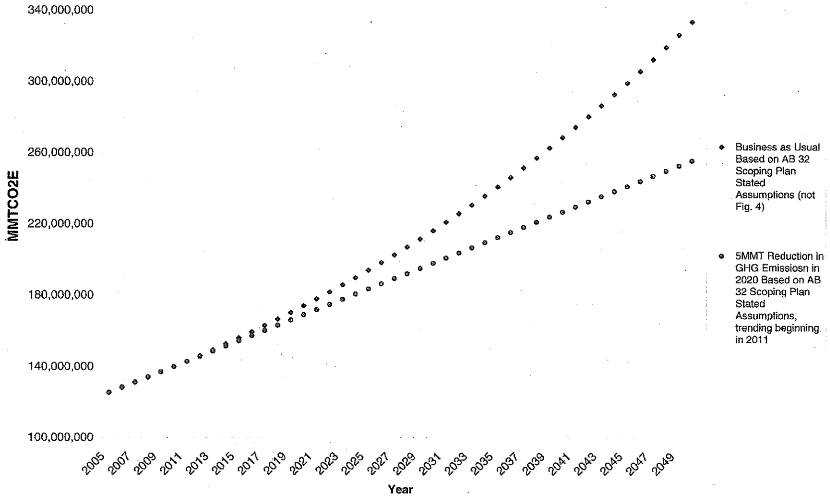
FIGURE 2 Change in Aggregate GHG Emissions from Land Use and Transportation Based Upon AB 32 Scoping Plan (Stated Assumptions)
