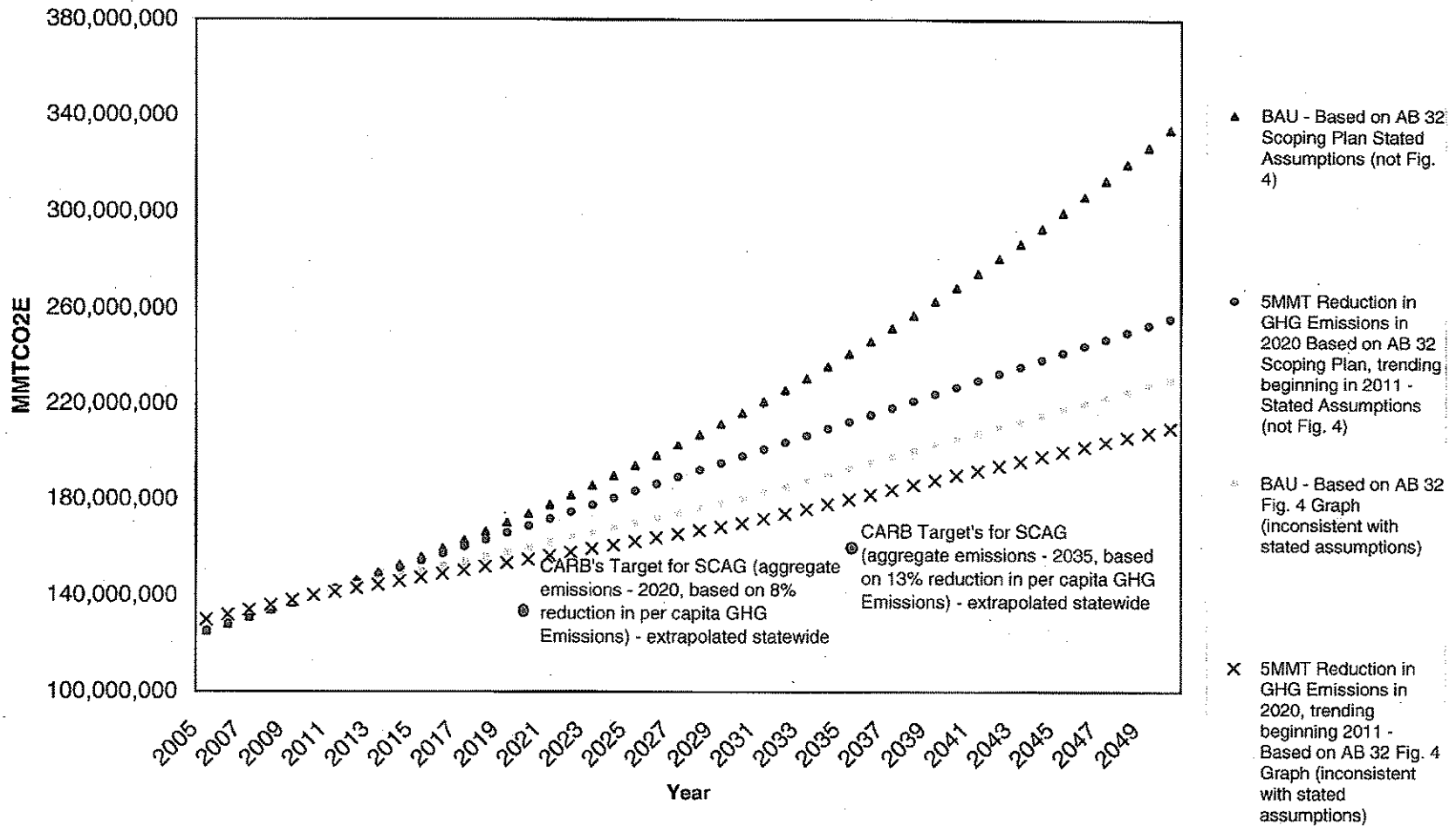
FIGURE 4 Change in Aggregate GHG Emissions from Land Use and Transportation Based Upon AB 32 Scoping Plan (Stated Assumptions vs. Fig. 4 Graph)
