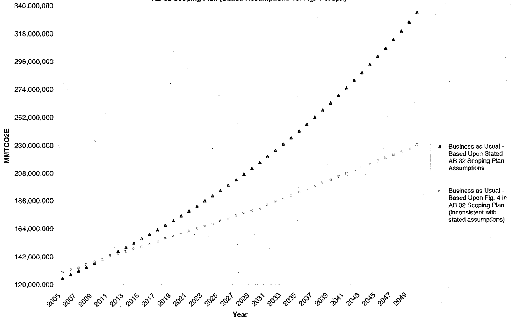
FIGURE 1 Business as Usual Comparison of the Change in Aggregate GHG Emissions from Land Use and Transportation Based Upon AB 32 Scoping Plan (Stated Assumptions vs. Fig. 4 Graph)
