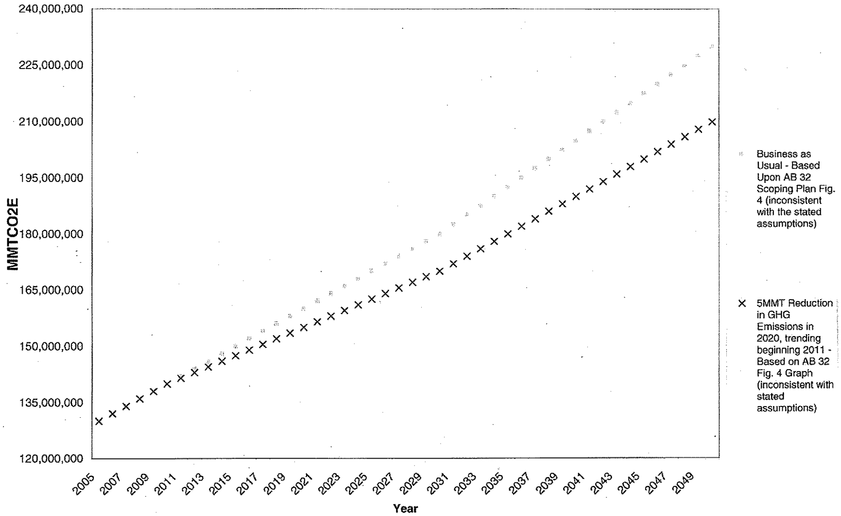
FIGURE 3 Change in Aggregate GHG Emissions from Land Use and Transportation Based Upon AB 32 Scoping Plan (Fig. 4 Graph)
