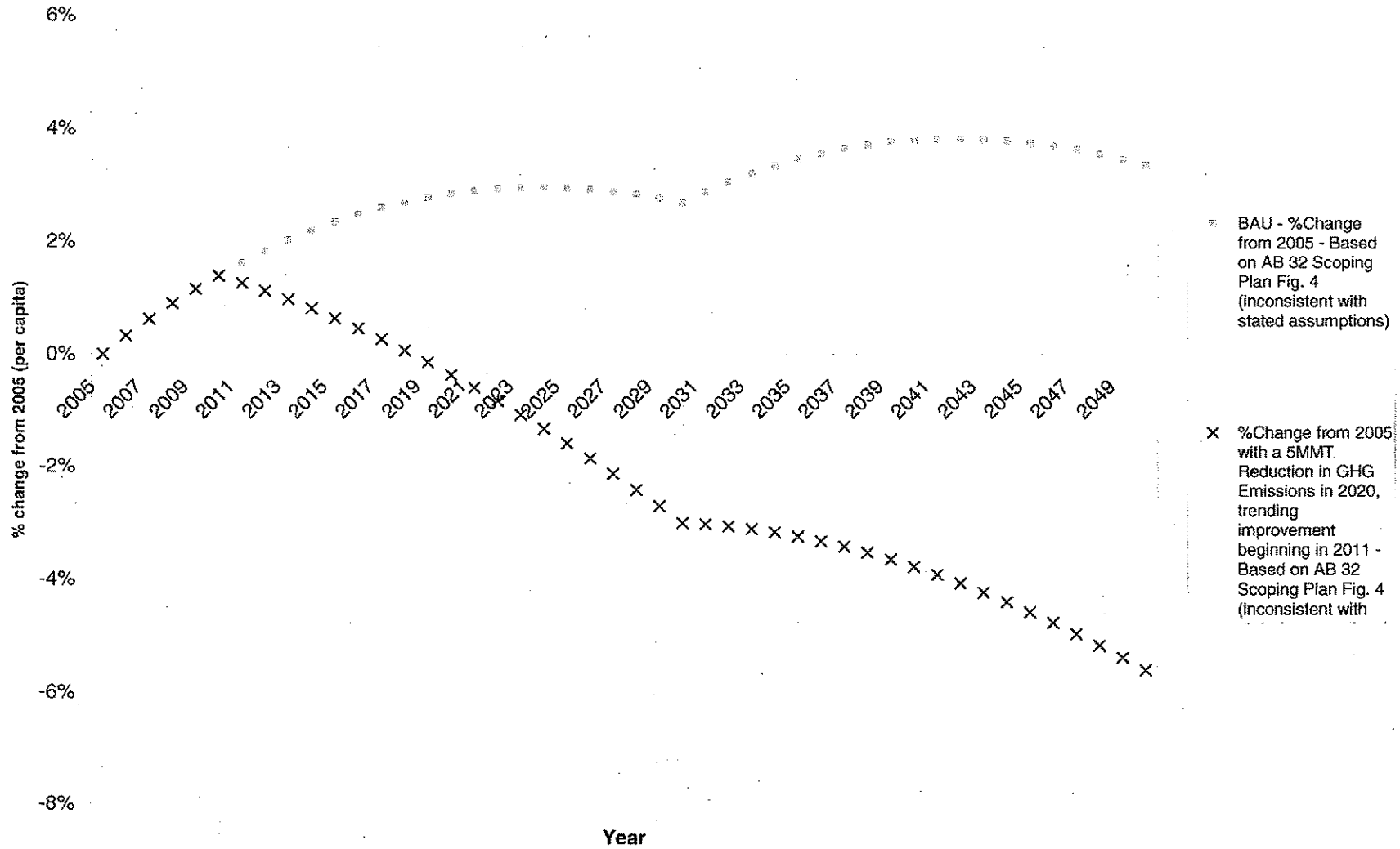
FIGURE 7 Percentage Change in Per Capita GHG Emissions - AB 32 Scoping Plan (Fig. 4 Graph)
