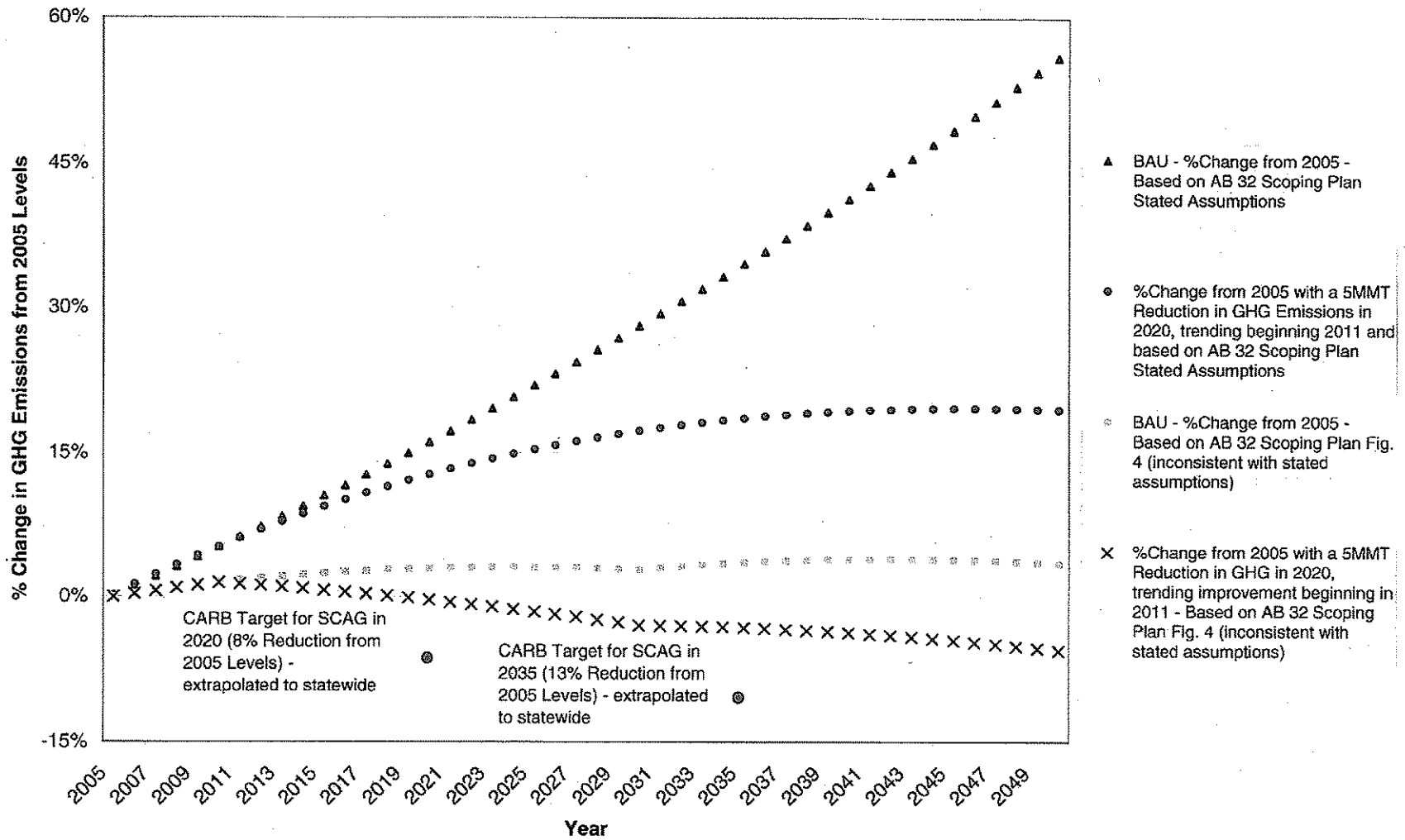
FIGURE 8 Percentage Change in Per Capita GHG Emissions - AB 32 Scoping Plan (Stated Assumptions vs. Fig. 4 Graph, assuming 2005 vehicles and fuels and a direct linear relationship between VMT and emissions)
