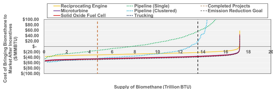
Figure 9. Biomethane Supply and Market Delivery Cost at LCFS and RIN Credit Prices of $200 and $1, Respectively
