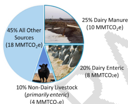
Figure 3. 2013 California Methane Emissions by Source
