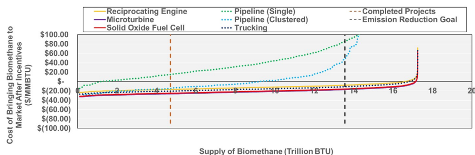
Figure 8. Biomethane Supply and Market Delivery Cost at LCFS and RIN Credit Prices of $150 and $0, Respectively
