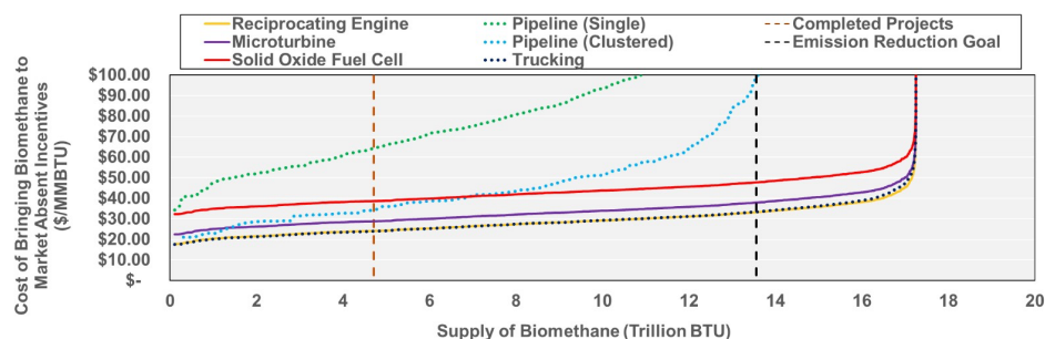
Figure 7. Biomethane Supply and Market Delivery Cost under Different Technology Options absent Federal and State Incentives
