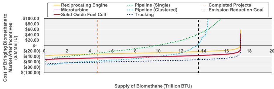
Figure 10. Biomethane Supply and Market Delivery Cost at LCFS and RIN Credits Prices of $200 and $2, Respectively
