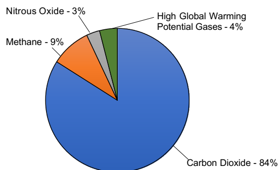
Figure 2. 2013 California GHG Emissions by Gas (Total 2013 Emissions~460 MMTCO 2 e)
