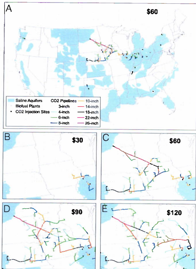
Fig. 3. Optimal capture, transportation, and sequestration networks for (A) sequestration credit of $60/tCO 2 at the scale of the United States and sequestration credits of (B) $30/tCO 2 , (C) $60/tCO 2 , (D) $90/tCO 2 , and (E) $120/tCO 2 focusing on the midwestern United States.
