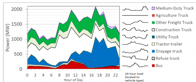
Projected CA On-Road Medium- and Heavy-Duty Vehicle Charging Load
