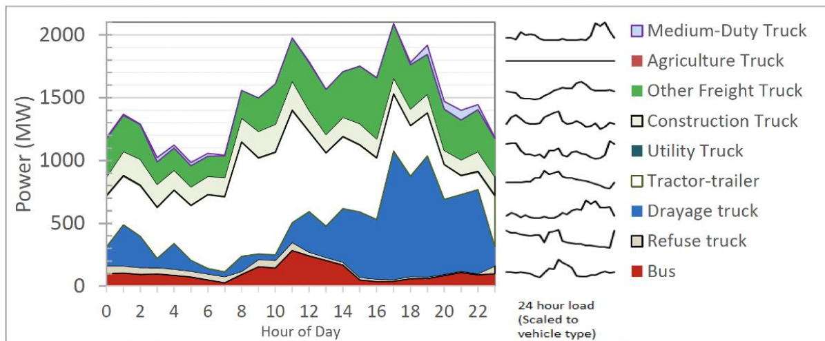
Projected CA On-Road Medium- and Heavy-Duty Vehicle Charging Load
