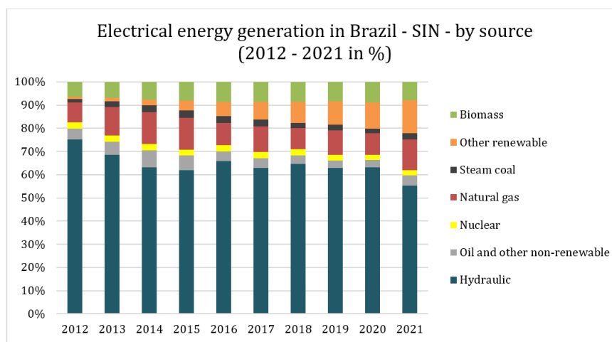
Figure 6. Electricity generation in Brazil by source (%). Source: EPE (2022).
