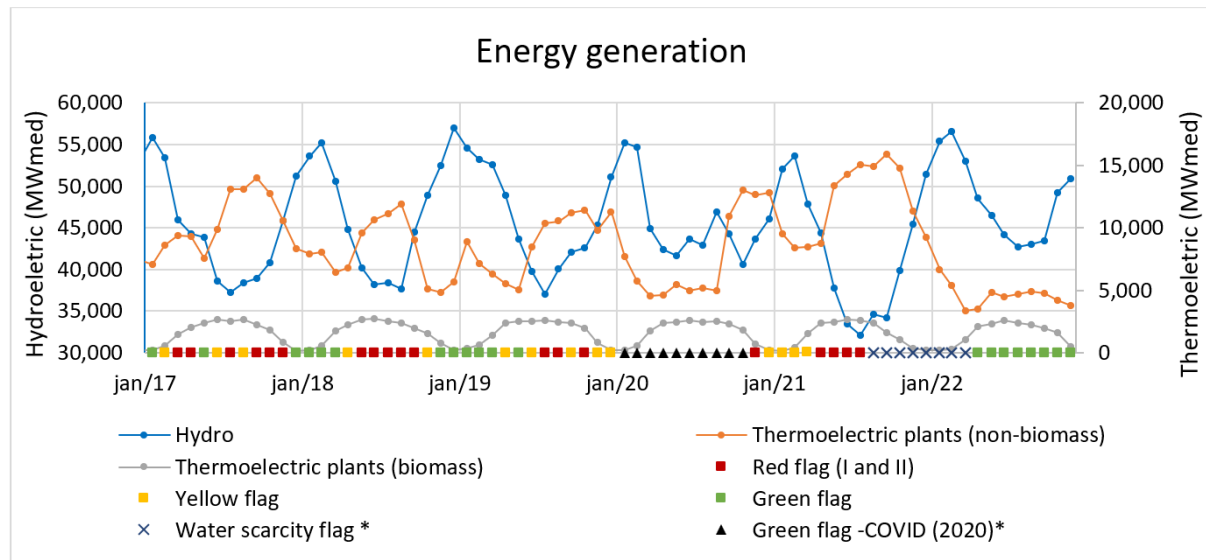
Figure 9. Monthly energy generation from hydroelectric and thermoelectric plants (using renewable sources “biomass”, and unrenewable sources “non-biomass”), and the monthly tariff flags from 2017 to 2022. Source: Agroicone, based on ONS (2023) 27 and ANEEL (2023b) 28 .
