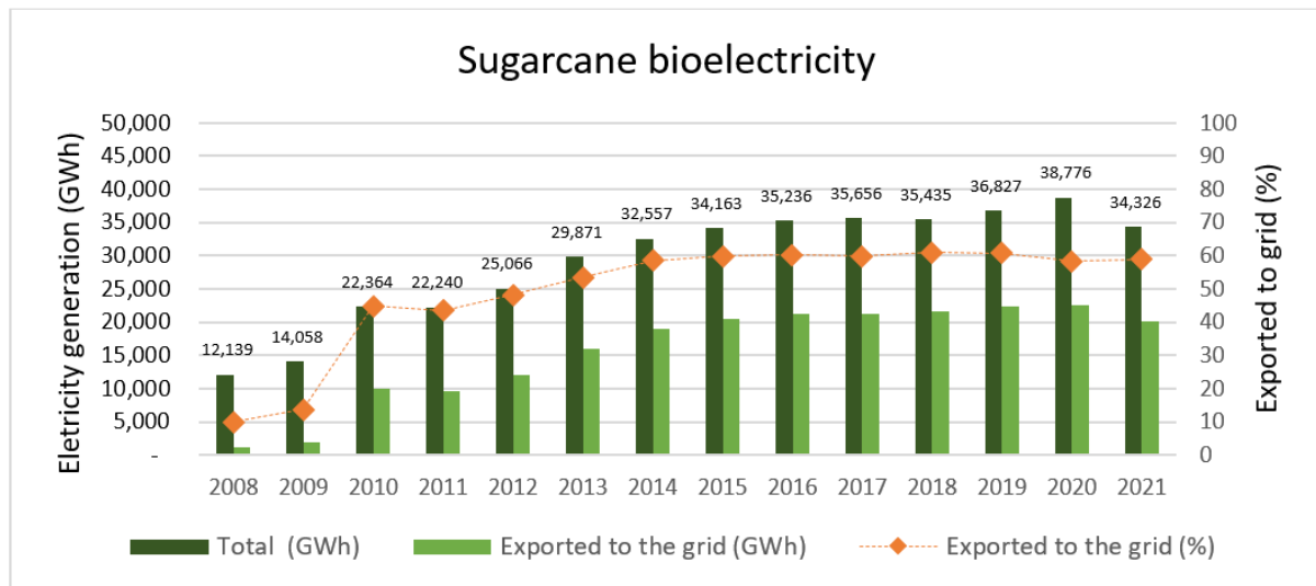
Figure 4. Electricity generation (GWh) from sugarcane bagasse since 2008. The reduction observed in 2021 is related to the hydrological crisis registered this year.
