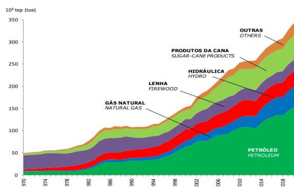
Figure 2. Primary energy production in Brazil from 1970 to 2021. Fonte: EPE (2022).
