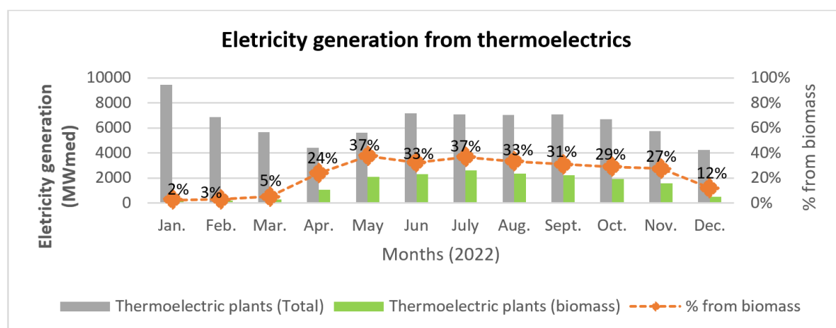
Figure 11. Electricity generation (MWmed) from thermoelectric plants, from all sources (total), and only from biomass. Percentage share of biomass in total thermoelectric generation in each month. Base year 2022. Source: Agroicone, based on ONS (2023) 36 .
