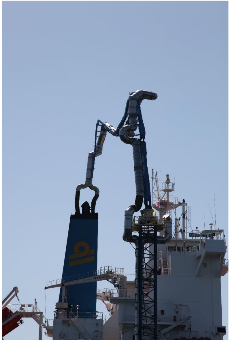
AMECS Barge System At-Anchor Direct-Connect Stack Exhaust Capture System
