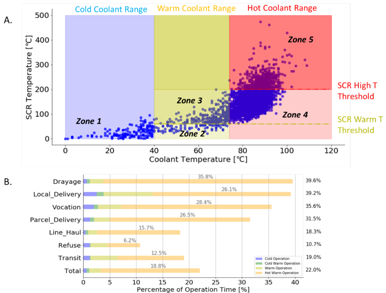
Figure 4. A) Number and type of engine start based on coolant temperature and SCR temperature. B) Percentage of time spent at different coolant-exhaust temperature conditions. Note: Engine starts defined as “cold” when coolant temp \leq 40^{\circ}\text{C} , warm-cold when coolant temp is between 40\text{--}75^{\circ}\text{C} and SCR temp is \leq 60^{\circ}\text{C} , warm when coolant temp is between 40\text{--}75^{\circ}\text{C} and SCR temp is between 60\text{--}200^{\circ}\text{C} , hot-warm when coolant temp is > 75^{\circ}\text{C} and SCR temp is \leq 200^{\circ}\text{C} , and hot when coolant temp is > 75^{\circ}\text{C} and SCR temp is > 200^{\circ}\text{C} .
