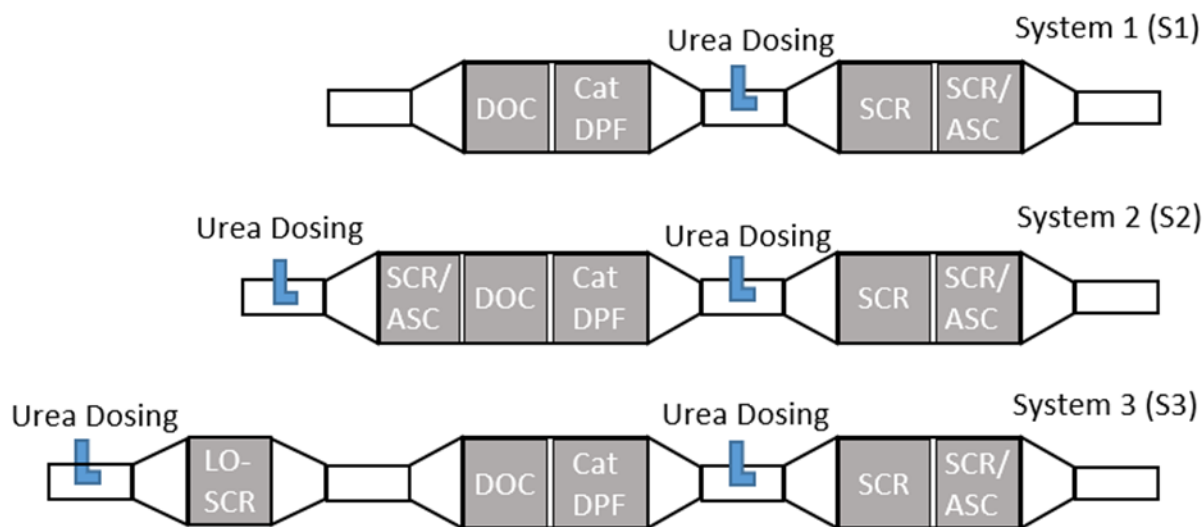
Figure 2. System configurations tested to demonstrate the feasibility of 2027 engine emissions.
