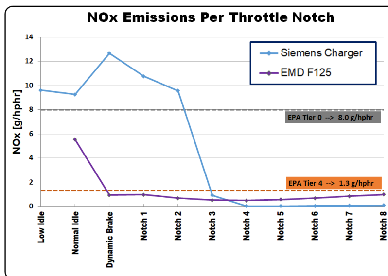
Figure 4 - NOx Emissions vs Power Setting
