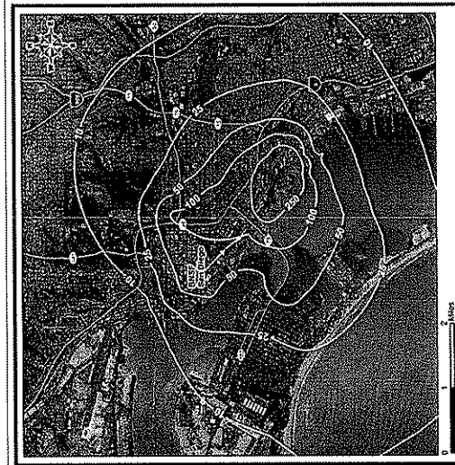
Cancer Risk Isopleth from Other Local Emission Sources
