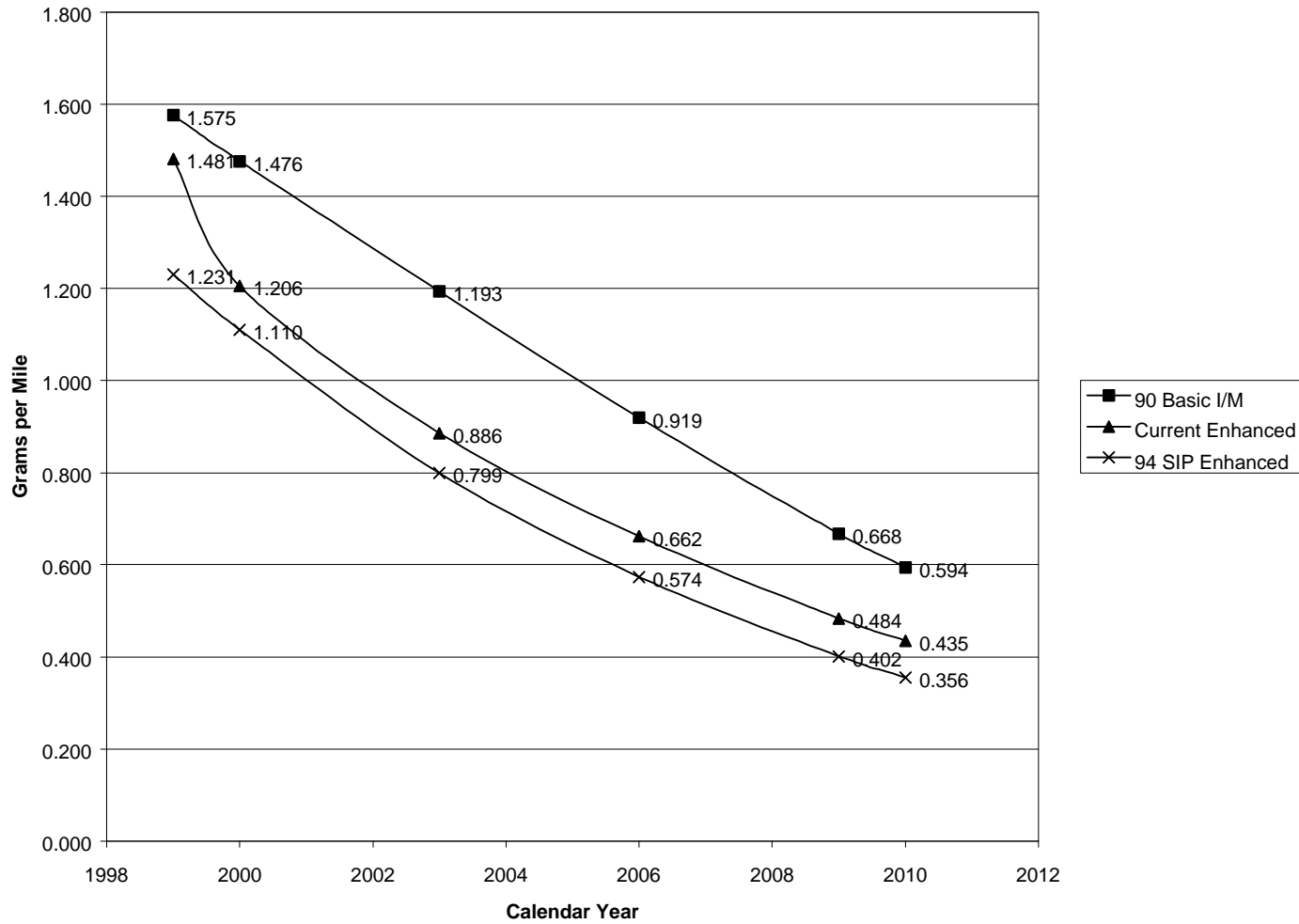
Medium-Duty Truck NOx Emission Rates, Draft EMFAC2000
