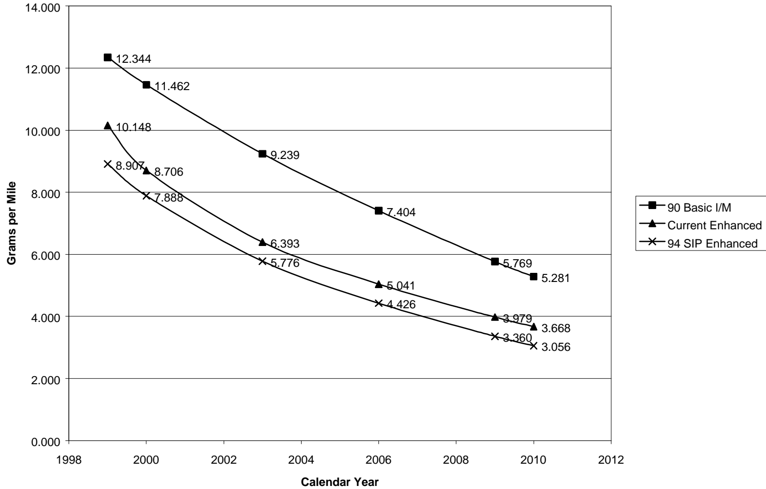
Light-Duty Truck CO Exhaust Emission Rates, Draft EMFAC2000
