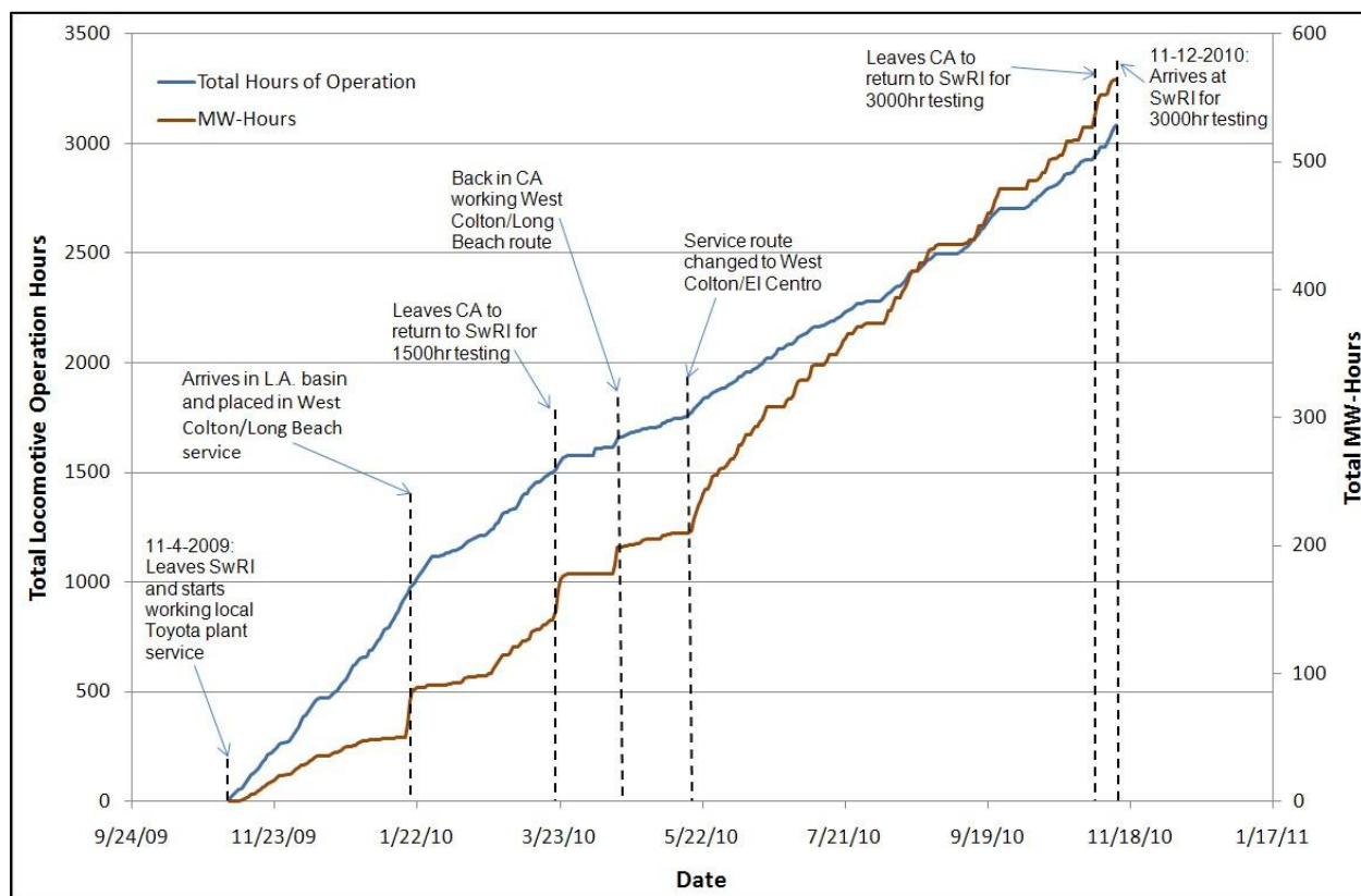
FIGURE 28. ENGINE HOUR AND MW-HOUR ACCUMULATION DURING FIELD DEMONSTRATION
