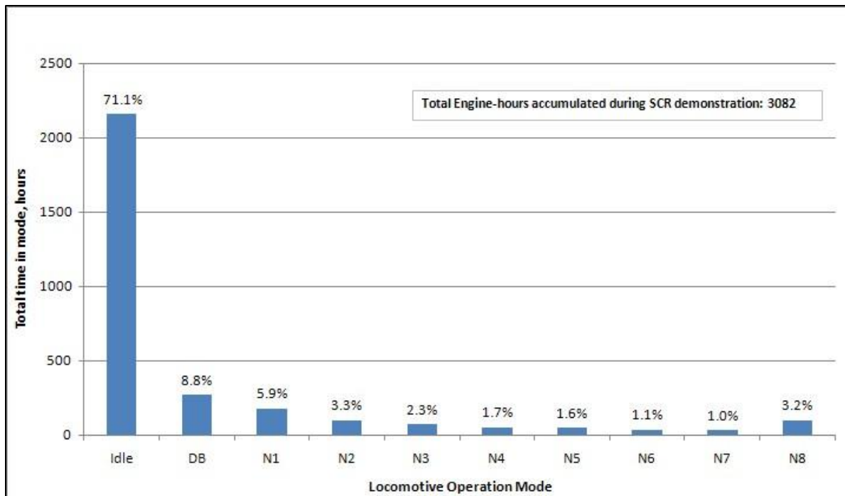
FIGURE 26. TOTAL TIME IN EACH OPERATING MODE AND RESULTING DUTY CYCLE DURING FIELD DEMONSTRATION
