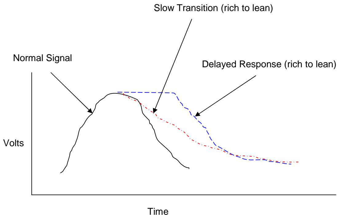
Fig. 1: O2 Sensor Deterioration Sketch
