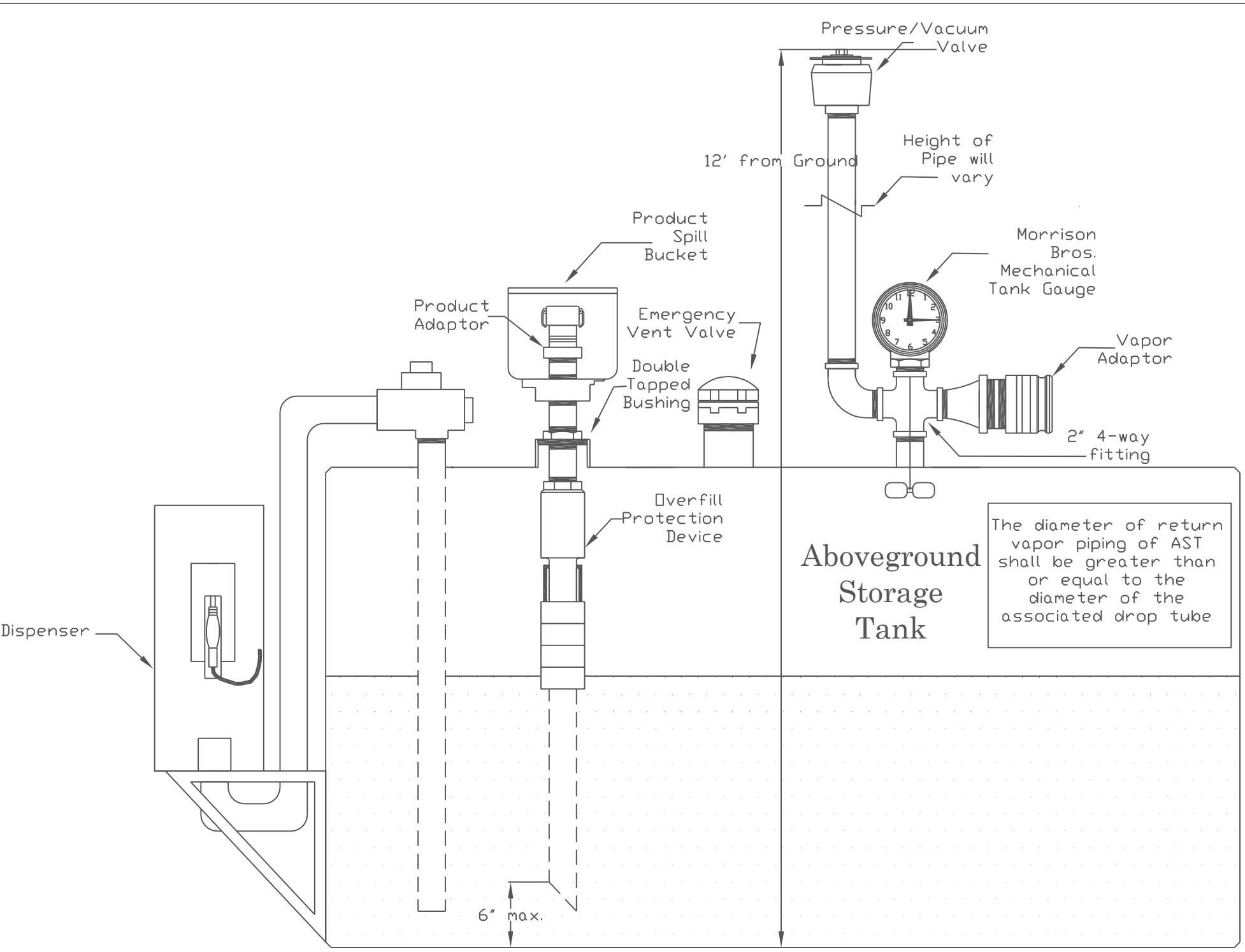
FAQ for AST: Figure 3: Alternate Phase I Installation Configuration
